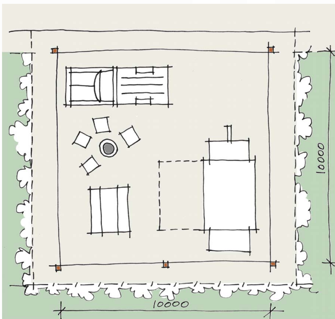
Car-based Campsite (Typical)
